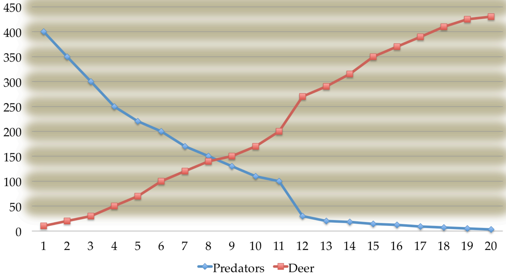
Ratio of predators and deer over time
