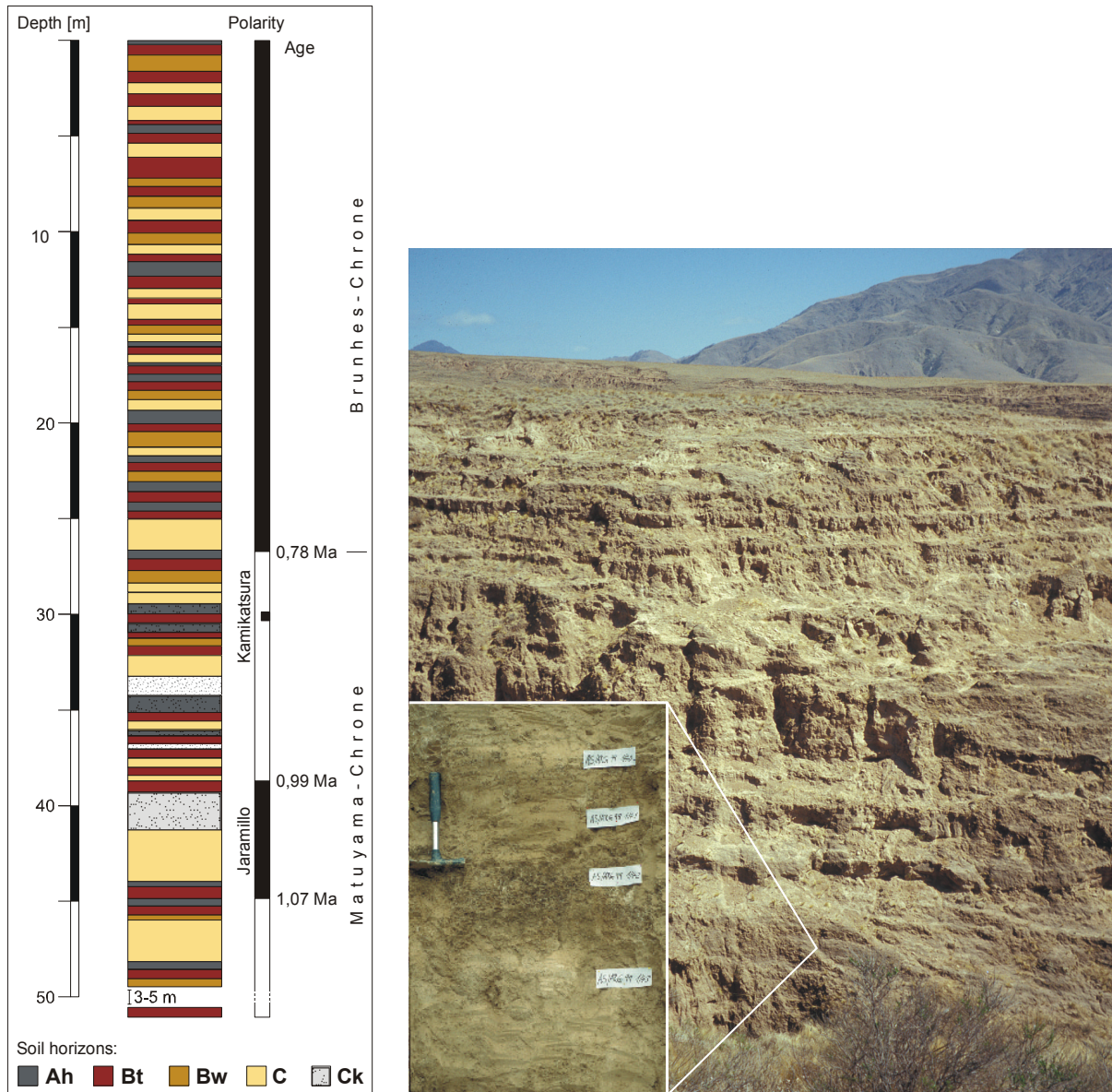
Fig 2: Abundant paleosol-loess sequences in the Andes of NW-Argentina (Valle de Tafi, 3000 m a.s.l.) with more than 31 paleosols. The zoom gives an example of a single paleosol. The profile reaches more than 1.2 million years back in time. Schellenberger et al 2003.
